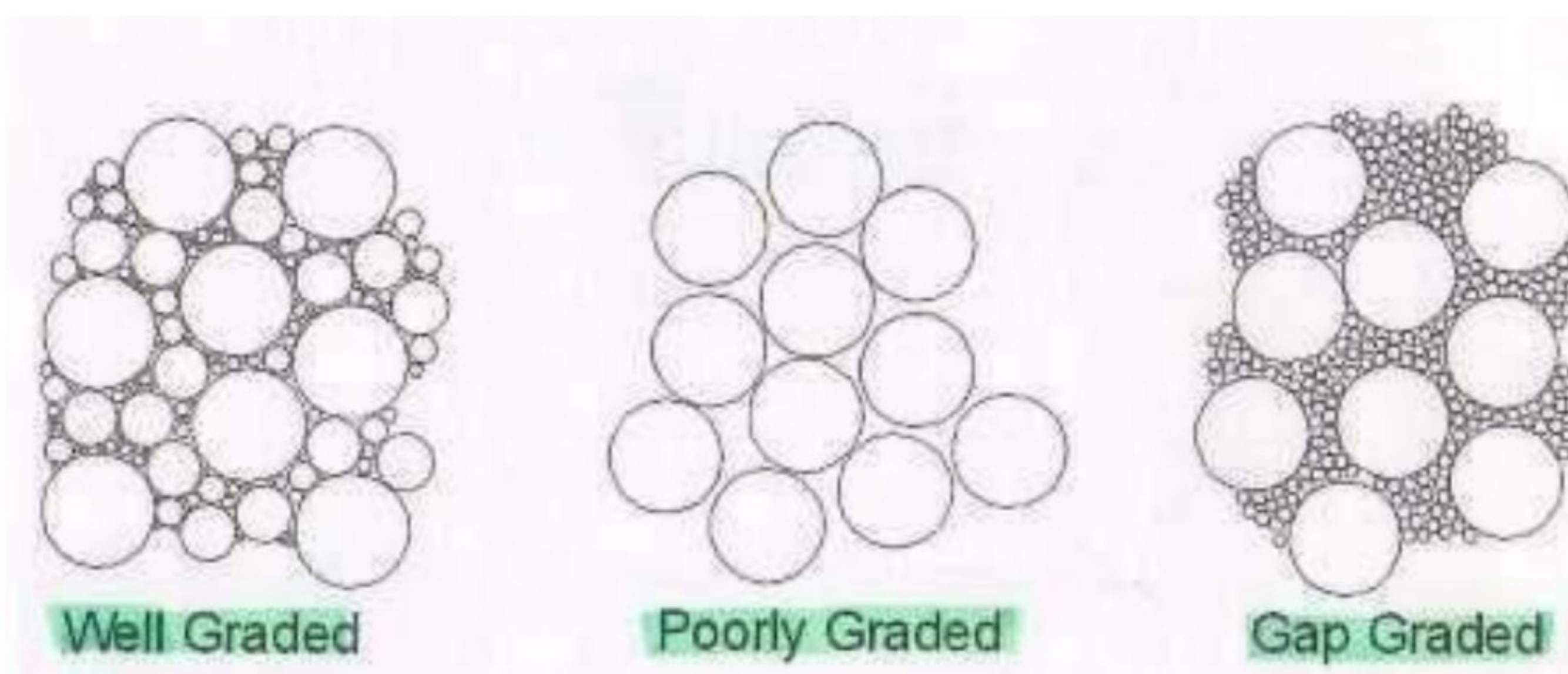
Fig.7: aggregate grading types
