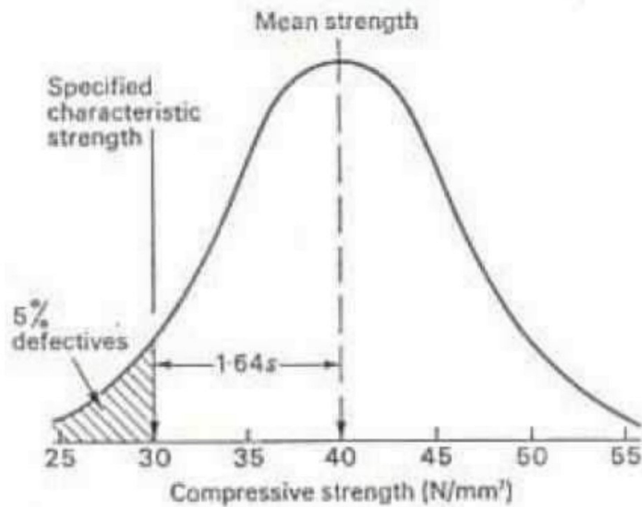
Fig.1: Means compressive strength vs characteristic compressive strength
